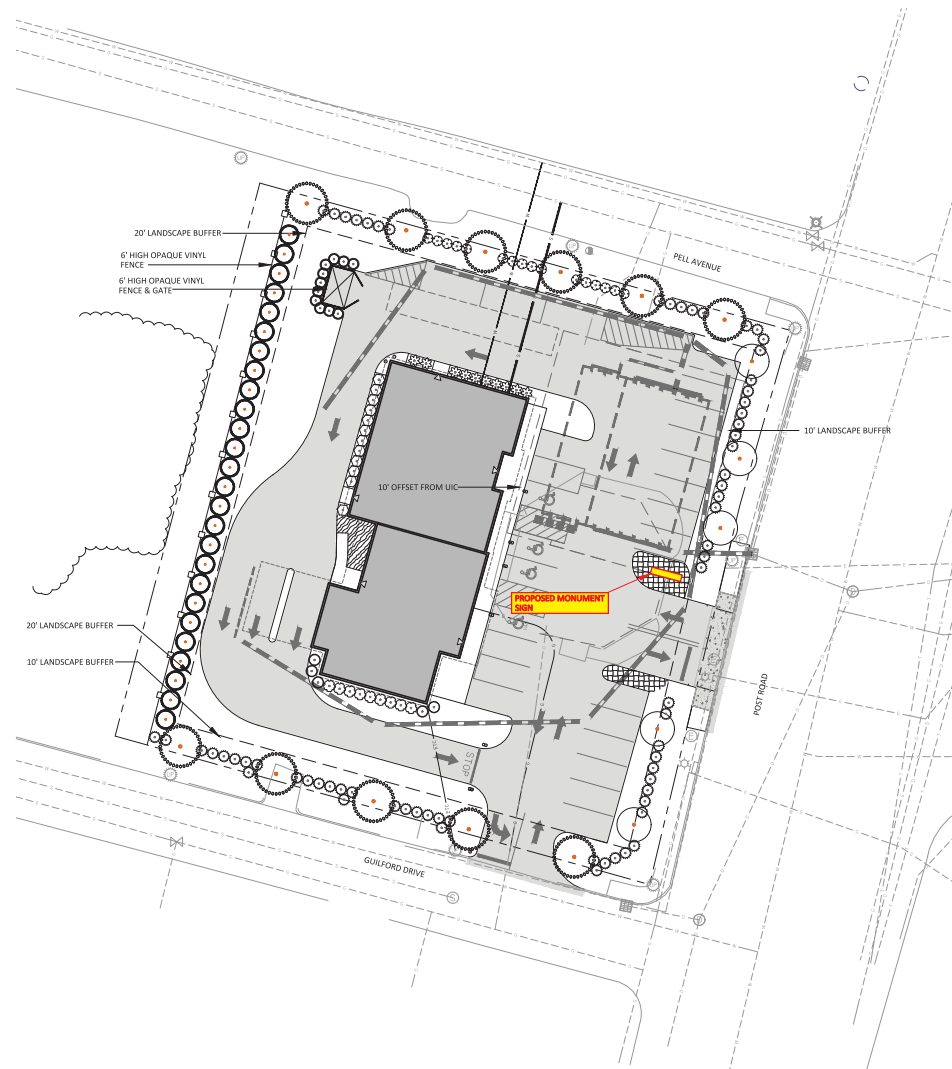
Landscape Plan
