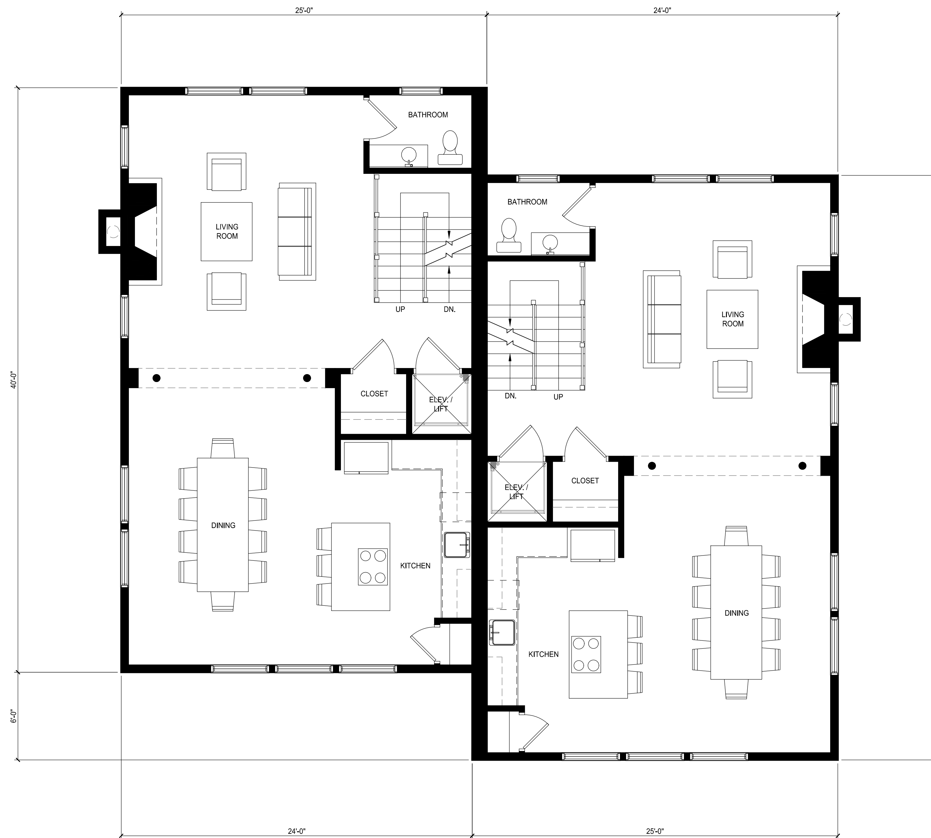
1 SECOND FLOOR PLAN 1/4" = 1'-0"
