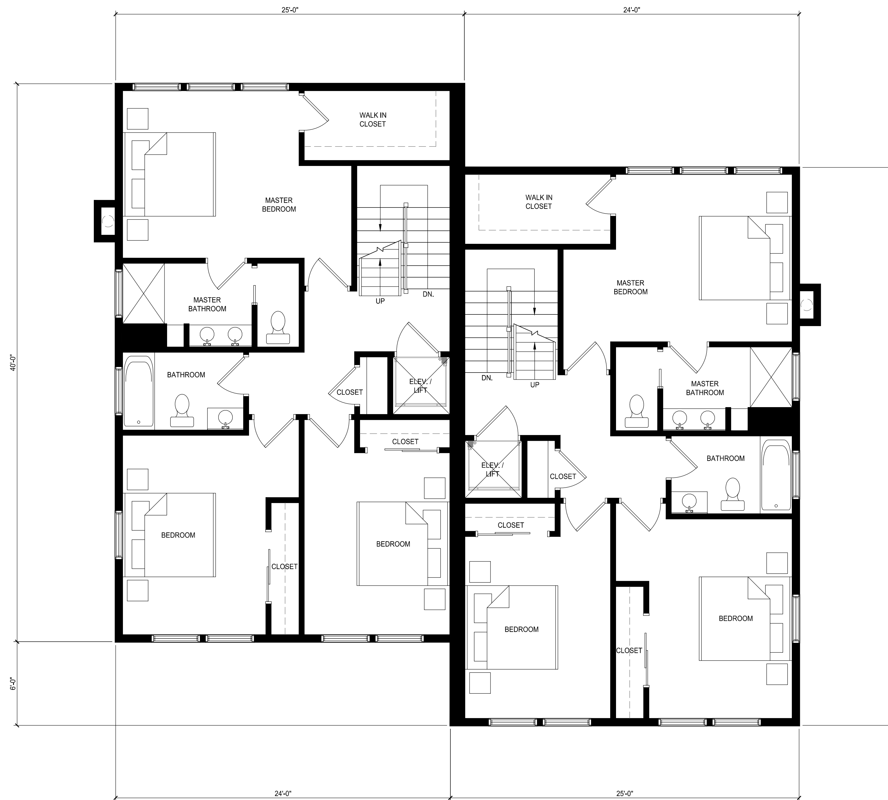
1 THIRD FLOOR PLAN 1/4" = 1'-0"
