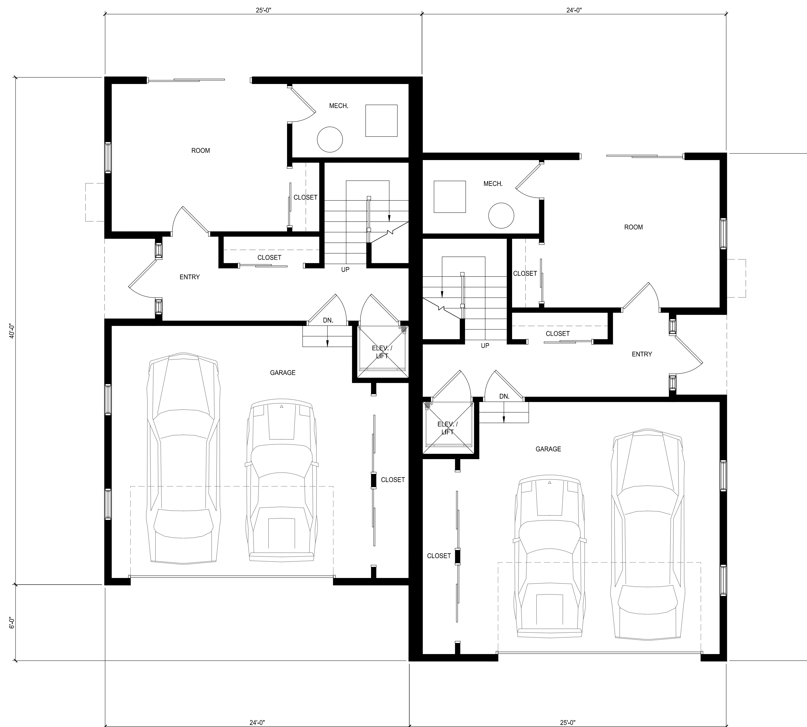
1 GROUND FLOOR PLAN 1/4" = 1'-0"
