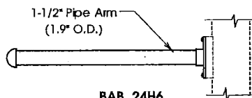
BAB 24H6 (banner arm, bolt-on, 24" lg., 1.5" \varnothing )
