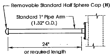
BAB 24H4 (banner arm, bolt-on, 24" lg., 1" \varnothing )
